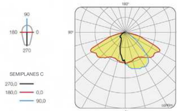
LRA-77700A1 | LED A1 82W POLAR DIAGRAM
