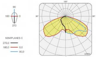
LRA-77700A3 | LED A3 37W POLAR DIAGRAM
